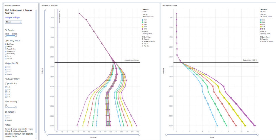
Sensitivity analysis visualization—hookload and torque analysis.
